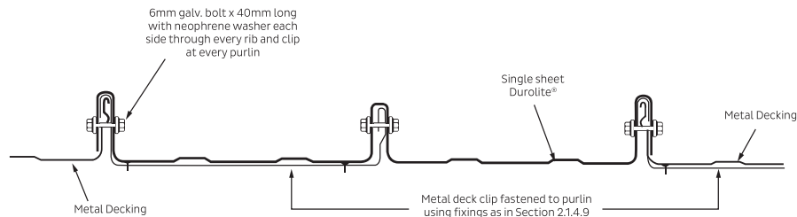
Fig 6 Detail For Single Durolite® Sheet With Dimondek® 400
