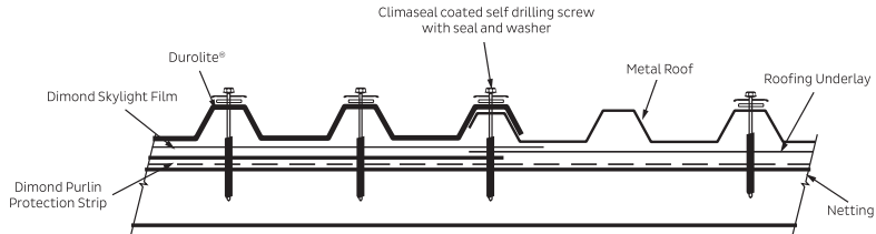
Fig 1 Dimond Skylight Film Detail
