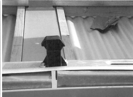
Dimondek® 630 clip installed to Purlins out of Alignment
