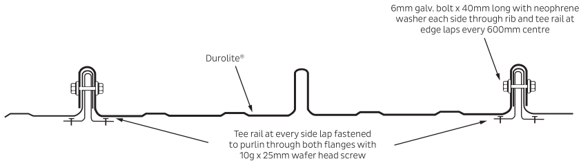
Fig 7 Multiple Durolite® Sheet Detail With Dimondek® 400
