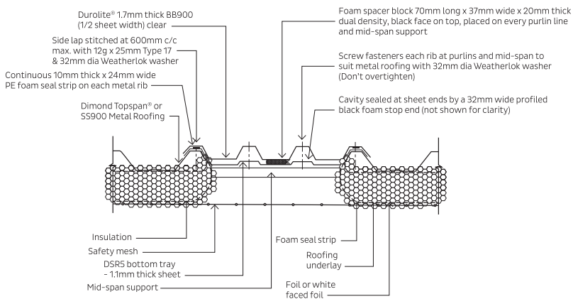
Fig 9 DSR5 Skylight Detail
