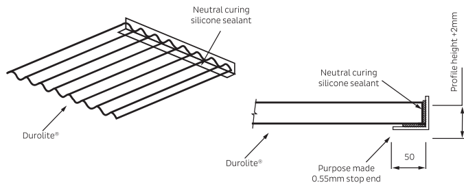
Fig 4 Stop End Detail
