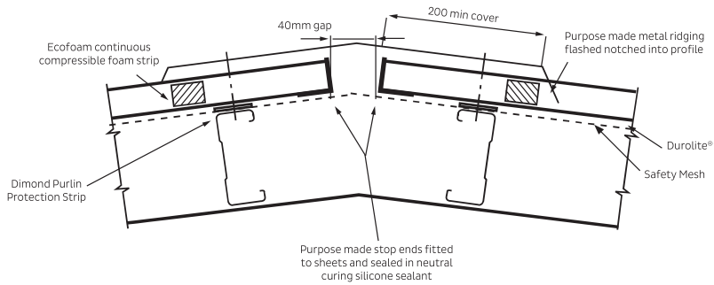
Fig 2 Ridge Detail
