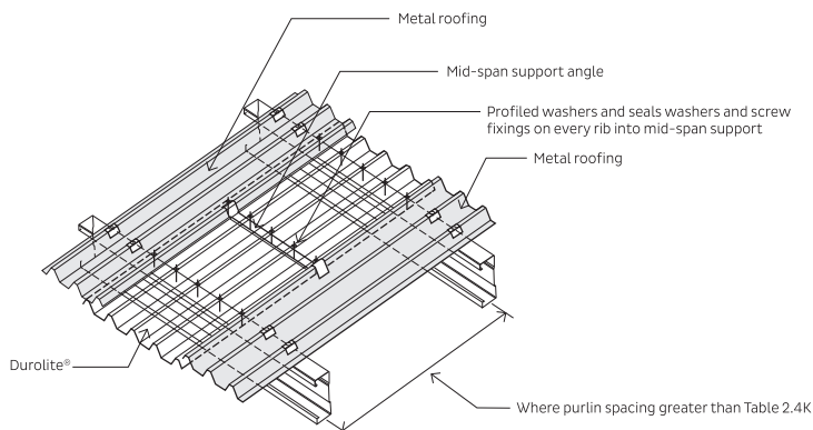
Fig 10 Mid-Span Support Detail (All Profiles Except Decking)
